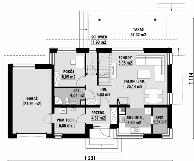
E-161 PARTER
