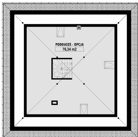
E-266b PODDASZE
