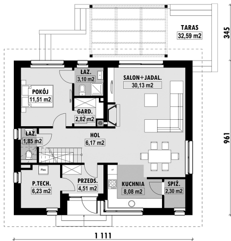
E-273a PARTER
